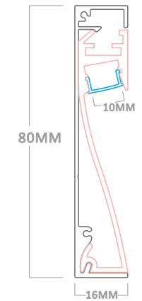
Skirting linear lighting
